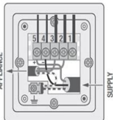
Wiring diagram - Mains Switching
