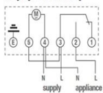
Wiring diagram - Mains Switching
